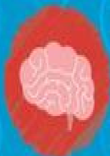
Anatomy
